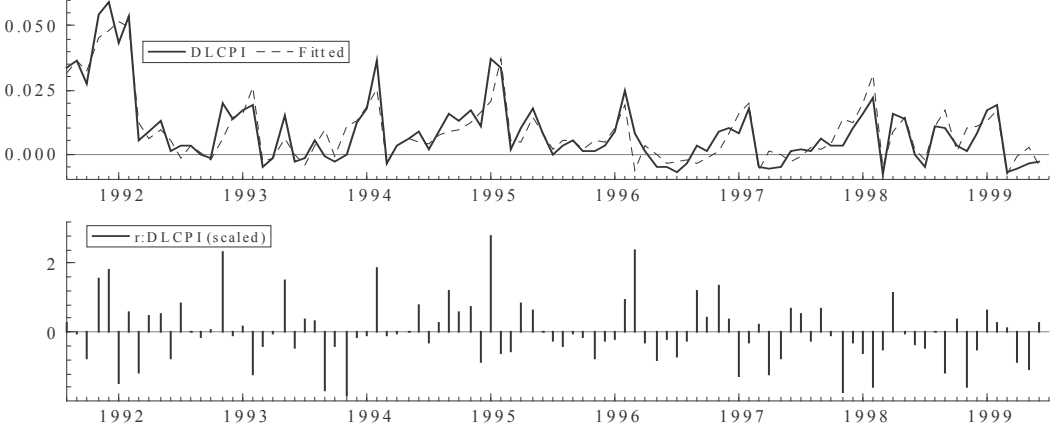
Fig. 3. Fitted and actual inflation rate and residuals.
